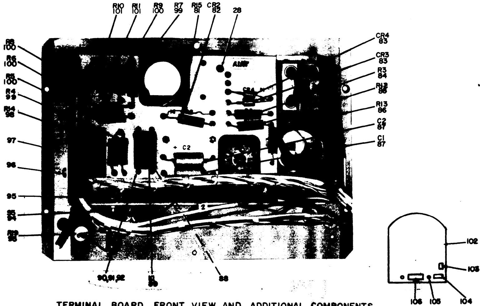
TERMINAL BOARD, FRONT VIEW AND ADDITIONAL COMPONENTS
