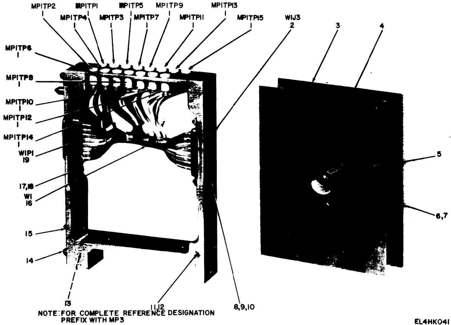
Figure 29. Extender, Module MX-4908/ARC-51X.
