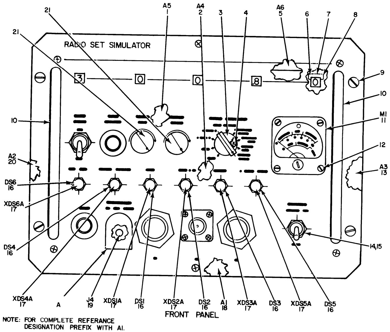
Figure 5. Simulators, Test Set, Radio SM-348/ARC-51X and SM-348A/ARC-51X (Sheet 1 of 3).
