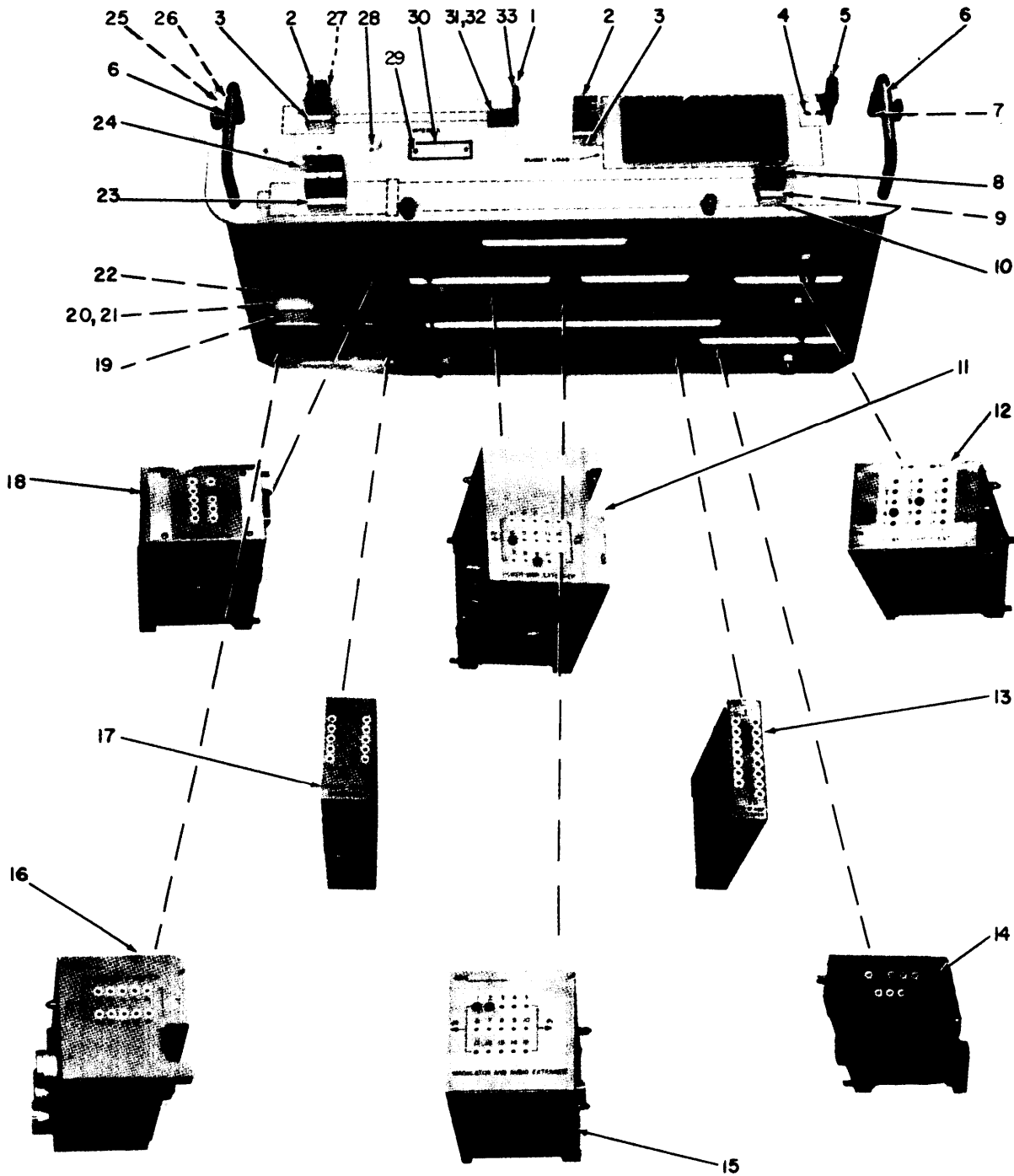
Figure 23. Mounting Tray, Module Extender MT-3372/ARC-51X.
