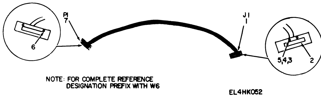
Figure 39. Cable Assembly, Special Purpose, Electrical CX-10187/ARC-51X.
