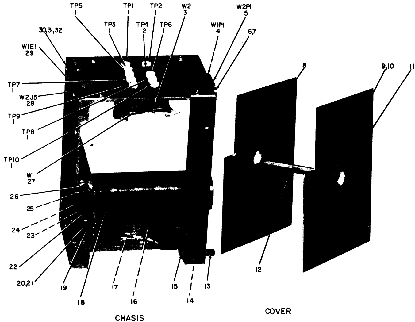
Figure 27. Extender, Module MX-4910/ARC-51X.
