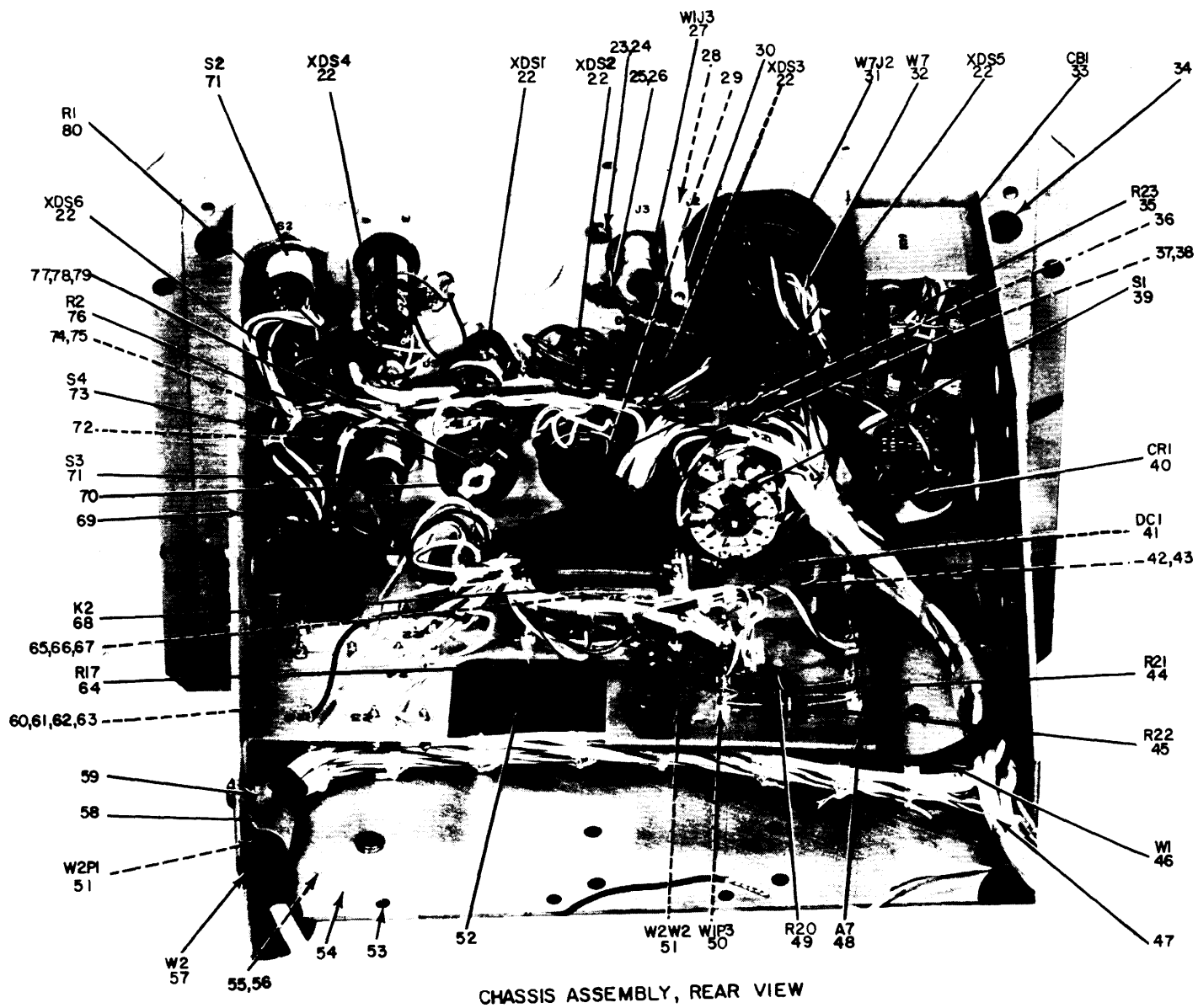
Figure 5. Simulators, Test Set, Radio SM-348/ARC-51X and SM-348A/ARC-51X (Sheet 2 of 3).
