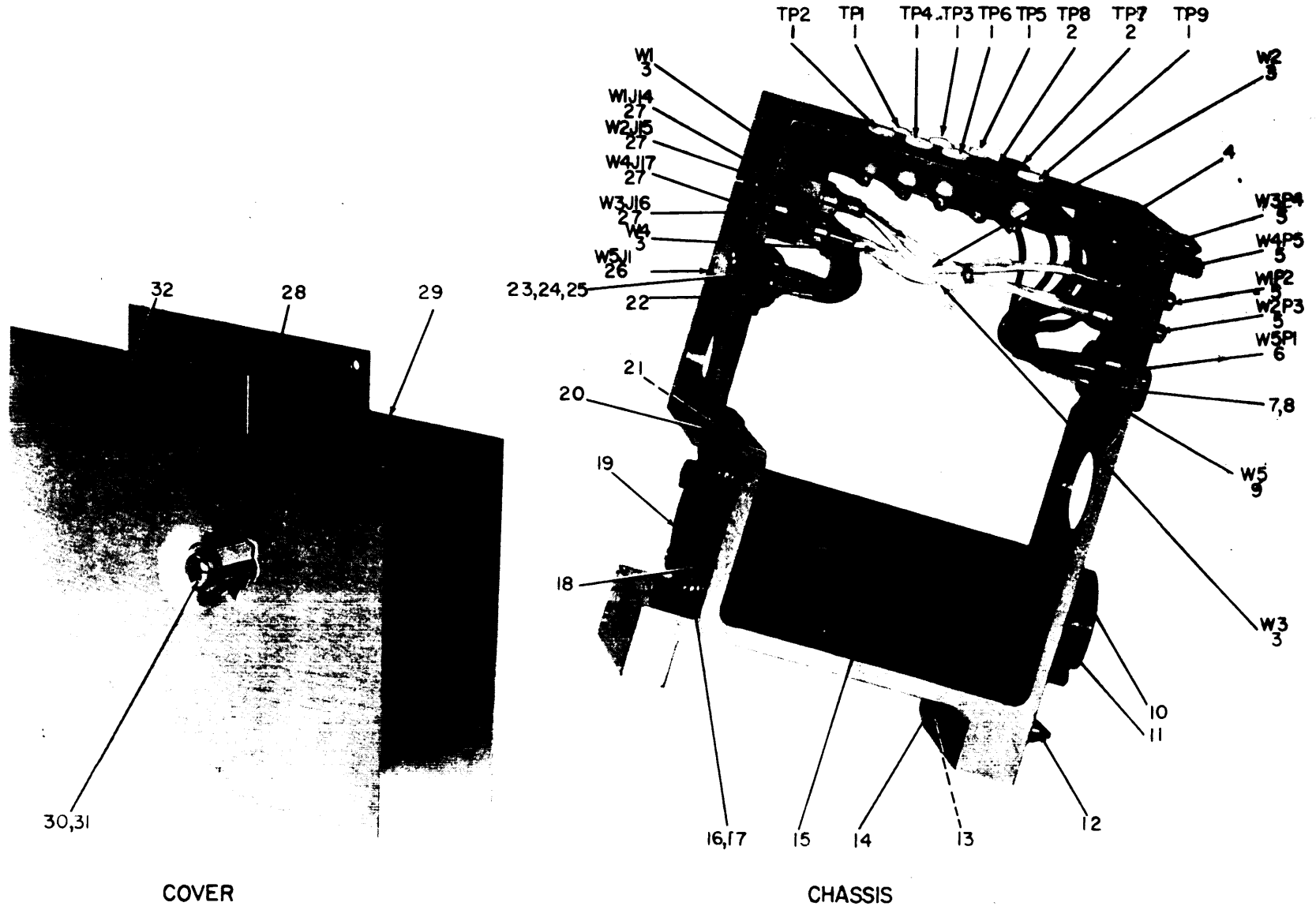
Figure 31. Extender, Module MX-4906/ARC-51X.
