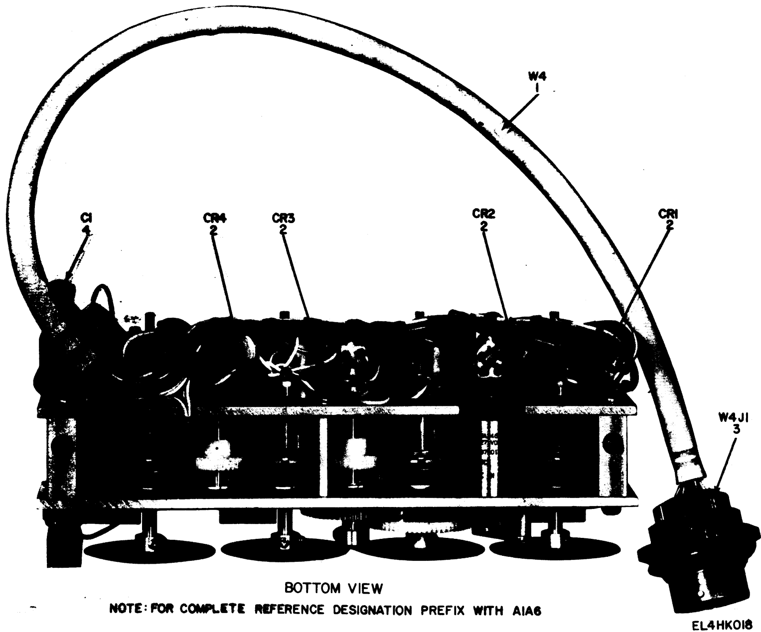
Figure 12. Readout Assembly (Sheet 1 of 2).
